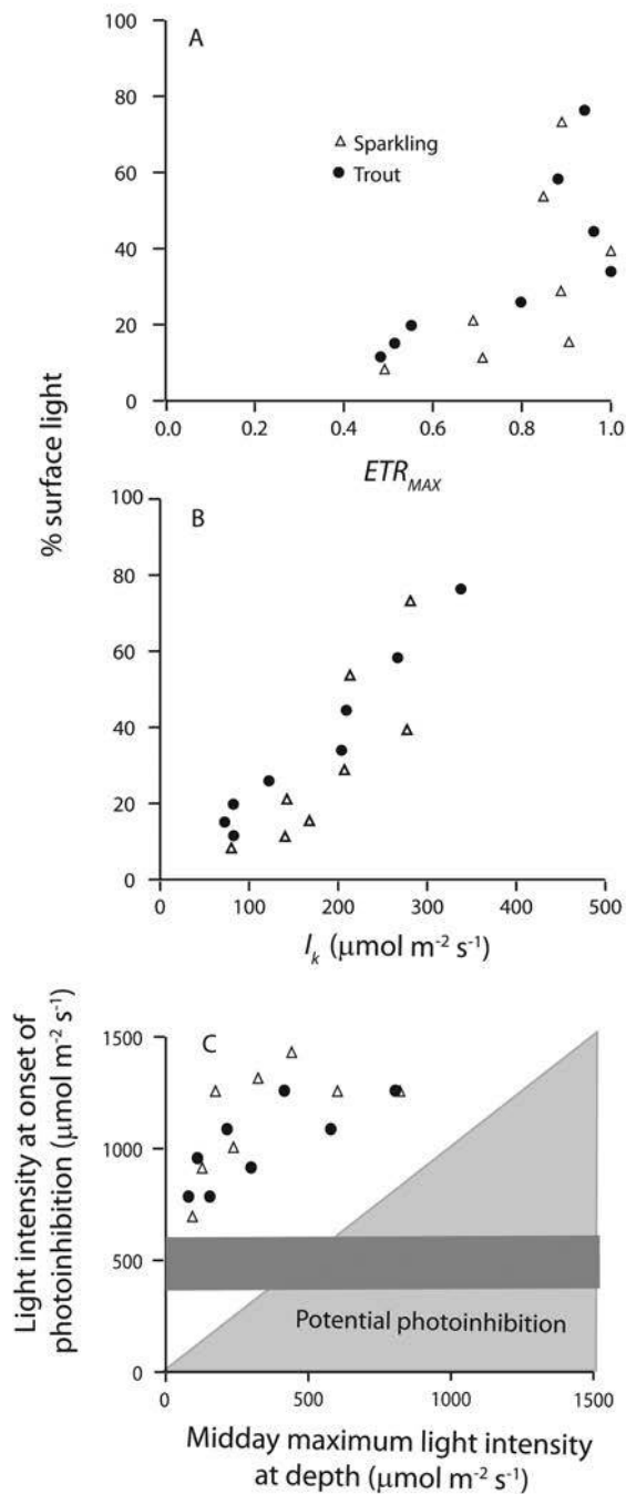
Figure 3. Photosynthesis–Irradiance (P–I) parameters derived from in situ pulse amplitude modulated (PAM) fluorometry on epipelon in Wisconsin (Sparkling and Trout Lakes). A.—Standardized maximum electron transfer rate ( ETR_{max} ). B.—Light intensity at onset of photosaturation ( I_k ) as a function of % surface light. C.—Relationship between light intensity at onset of photoinhibition estimated from the PAM P–I curves as a function of the maximum light intensity that periphyton experience at depth they occur. The grey bar denotes the range of light intensities at which phytoplankton from the 2 lakes exhibited photoinhibition. Each point represents epipelon measured at a single depth.
